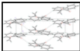
Fig. 2. Packing diagram of the title compound, viewed down the a axis. Dashed lines indicate weak intermolecular C—H...O hydrogen bonds.
